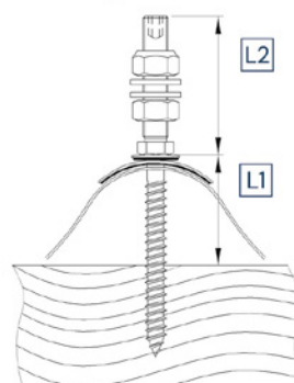
Bølgepap af fibercement Corrugated fibre cement
