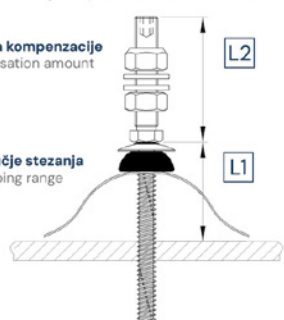
Valoviti profil i sendvič element Corrugated profile and sandwich element
