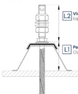
Trapezoidni profil i sendvič element Trapeze profile and sandwich element
