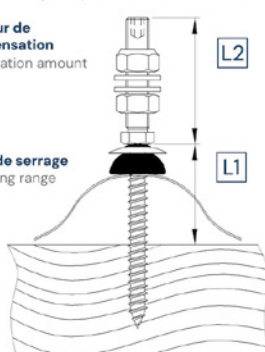
Profilé ondulé et élément sandwich Corrugated profile and sandwich element
