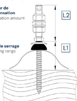
Profilé ondulé et élément sandwich Corrugated profile and sandwich element
