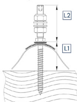
Ciment ondulé Corrugated fibre cement
