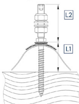
Korrugerad fibercement Corrugated fibre cement
