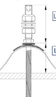
Cement falisty włóknisty Corrugated fibre cement
