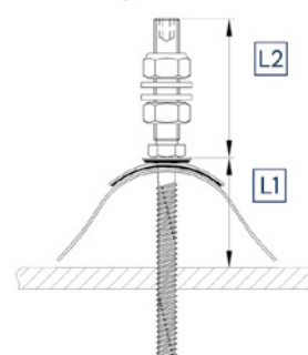
Cement falisty włóknisty Corrugated fibre cement
