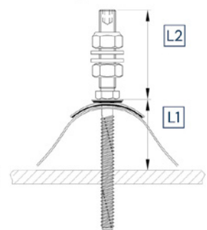
Oluklu fiber çimento Corrugated fibre cement
