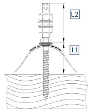
Oluklu fiber çimento Corrugated fibre cement
